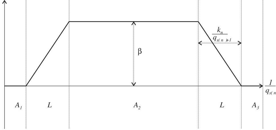
FIGURE 2. The function \psi_n on [0, q_{s(n)}^{-1}] . A_i and L are defined in Definition 5.
