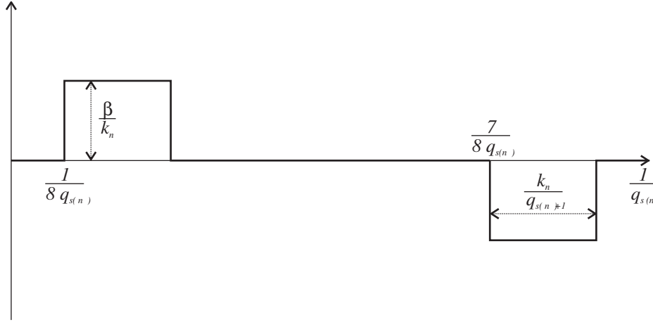
FIGURE 1. The function \varphi_n on [0, q_{s(n)}^{-1}] . \varphi_n is 0 on the rest of \mathbb{T}^1 .
